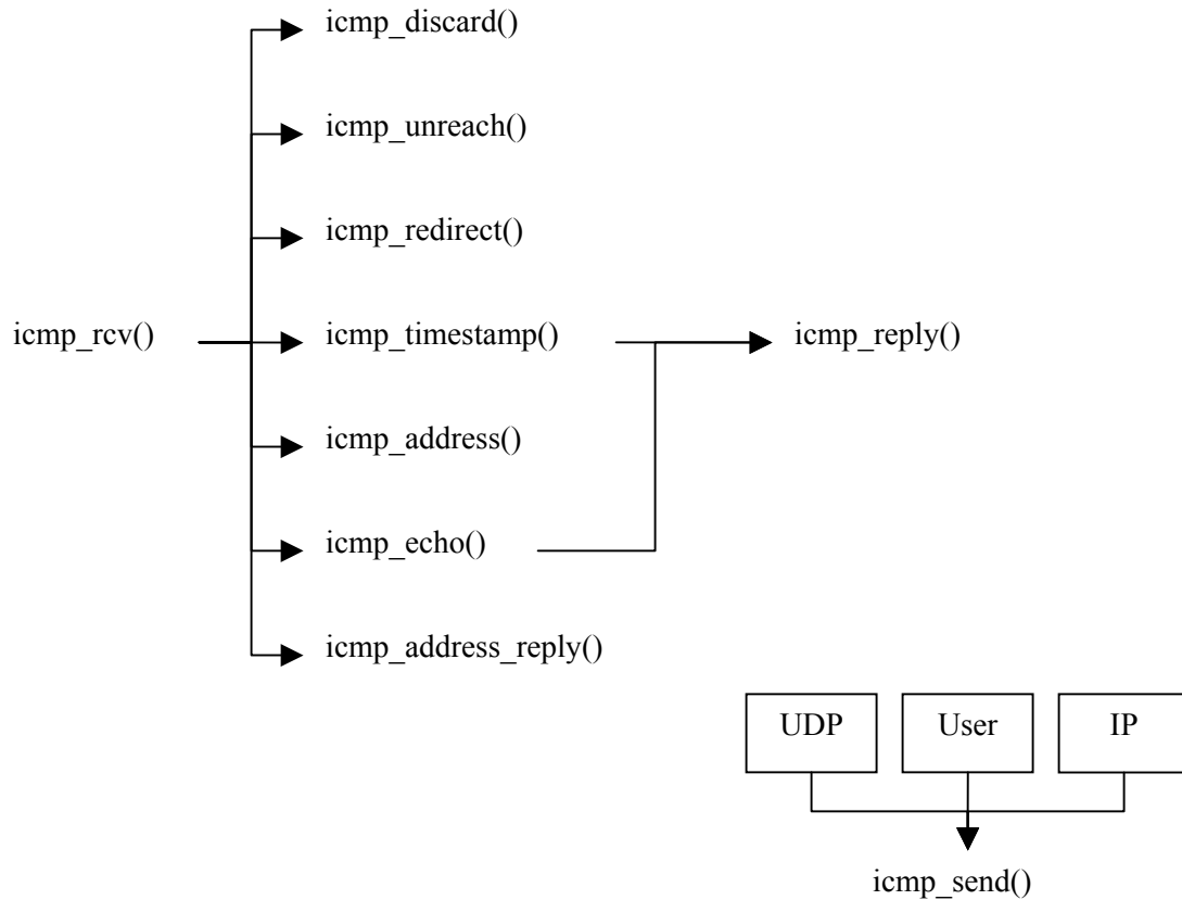
Figure 9: ICMP functions
