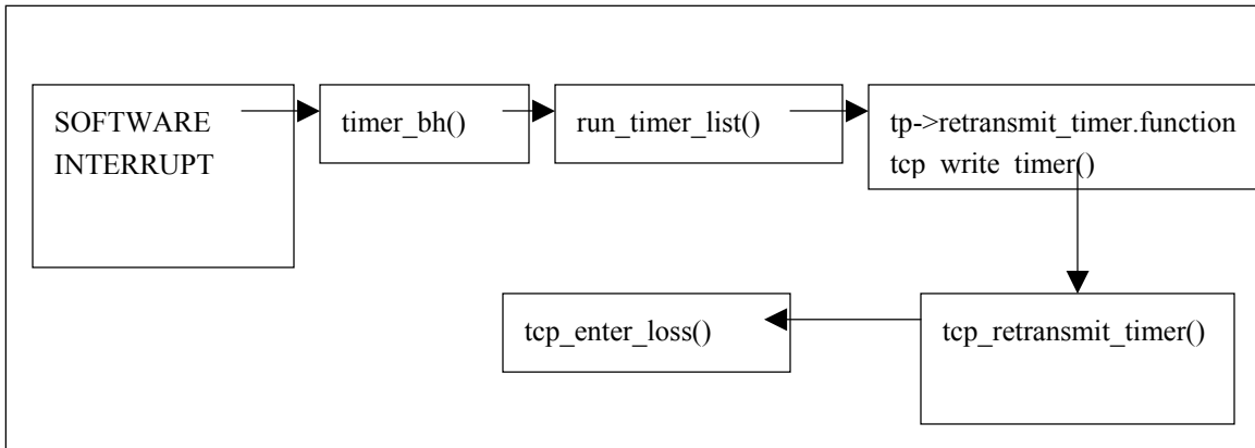
Figure 14: Timeout arrival
